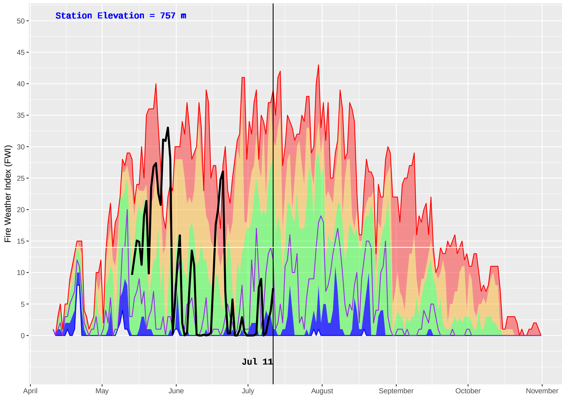
DOWNIE (905) : Historical (2005–2016) and Current (2018) Noon Fire Weather Index (FWI)
