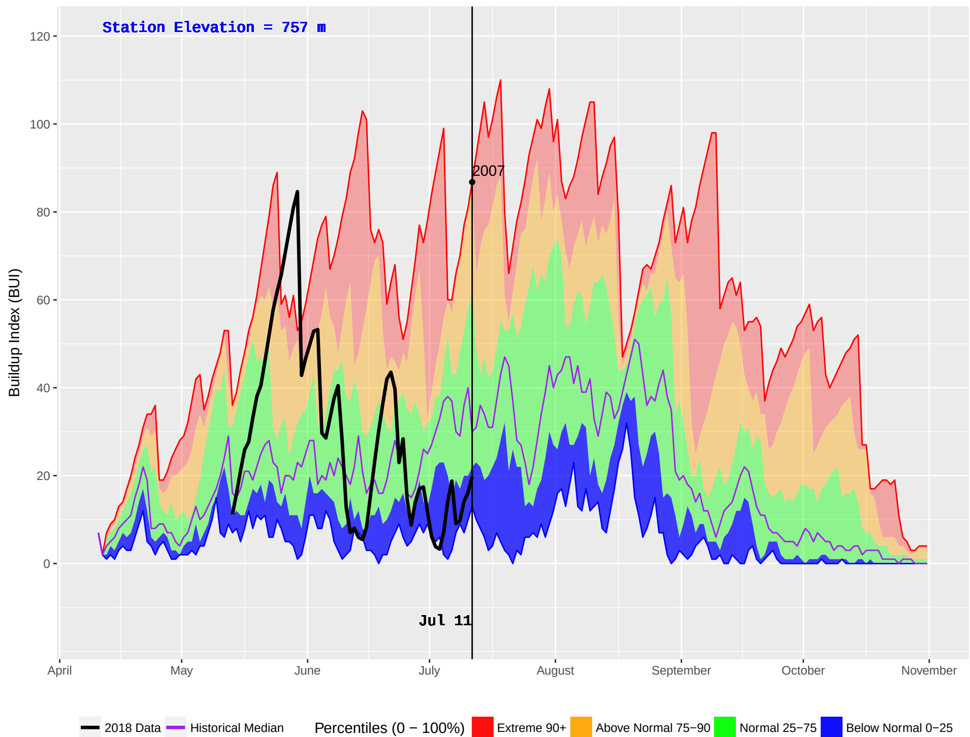
DOWNIE (905) : Historical (2005–2016) and Current (2018) Noon Buildup Index (BUI)
